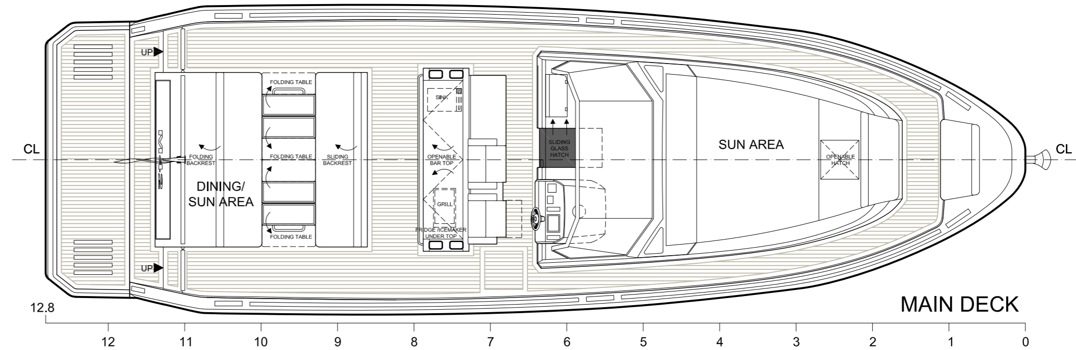
12 11 10 9 8 7 6 5 4 3 2 1 0 TOP VIEW
